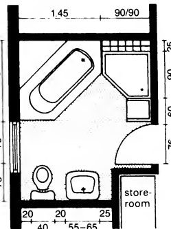
⑧ Corner bath and shower
